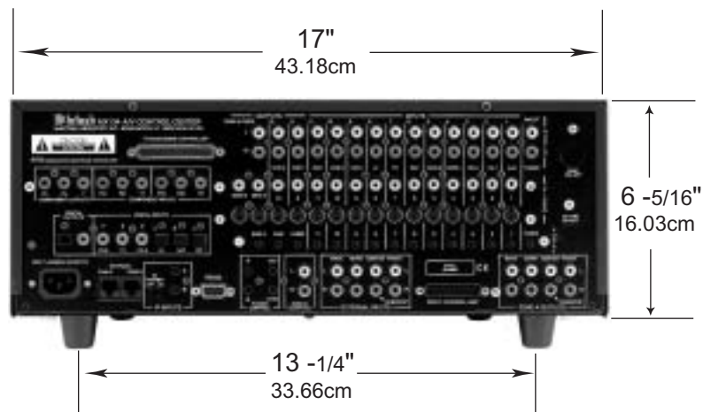
Rear View of the MX134
