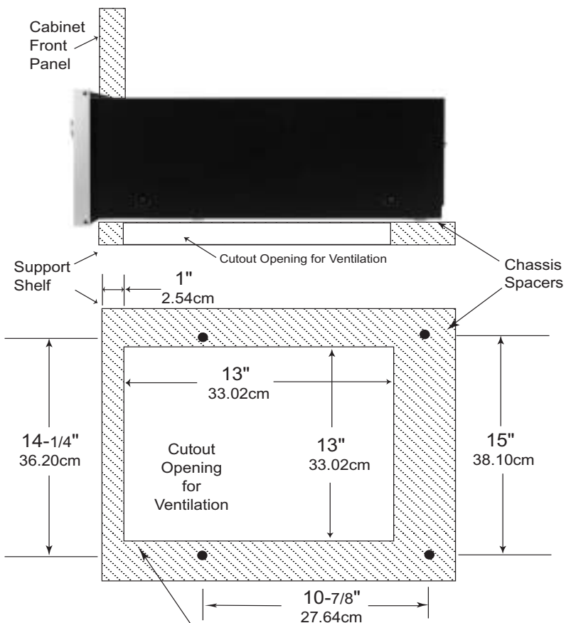
MX134 Bottom View in Custom Cabinet
