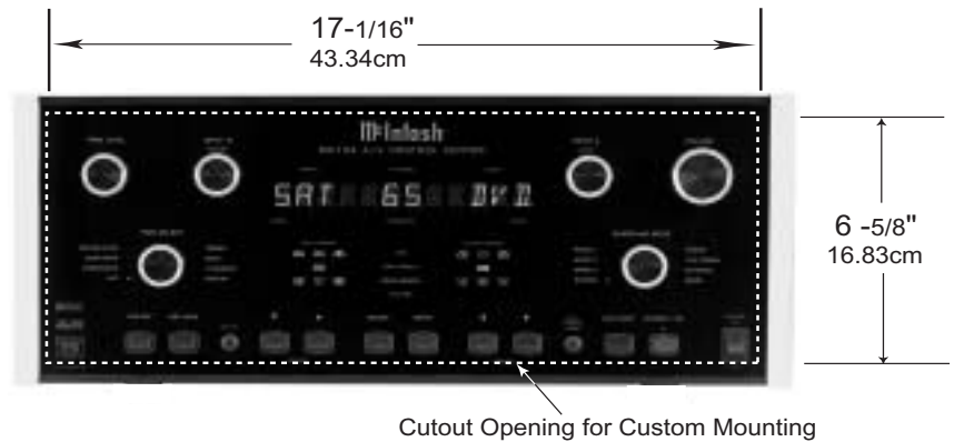
MX134 Front Panel Custom Cabinet Cutout
